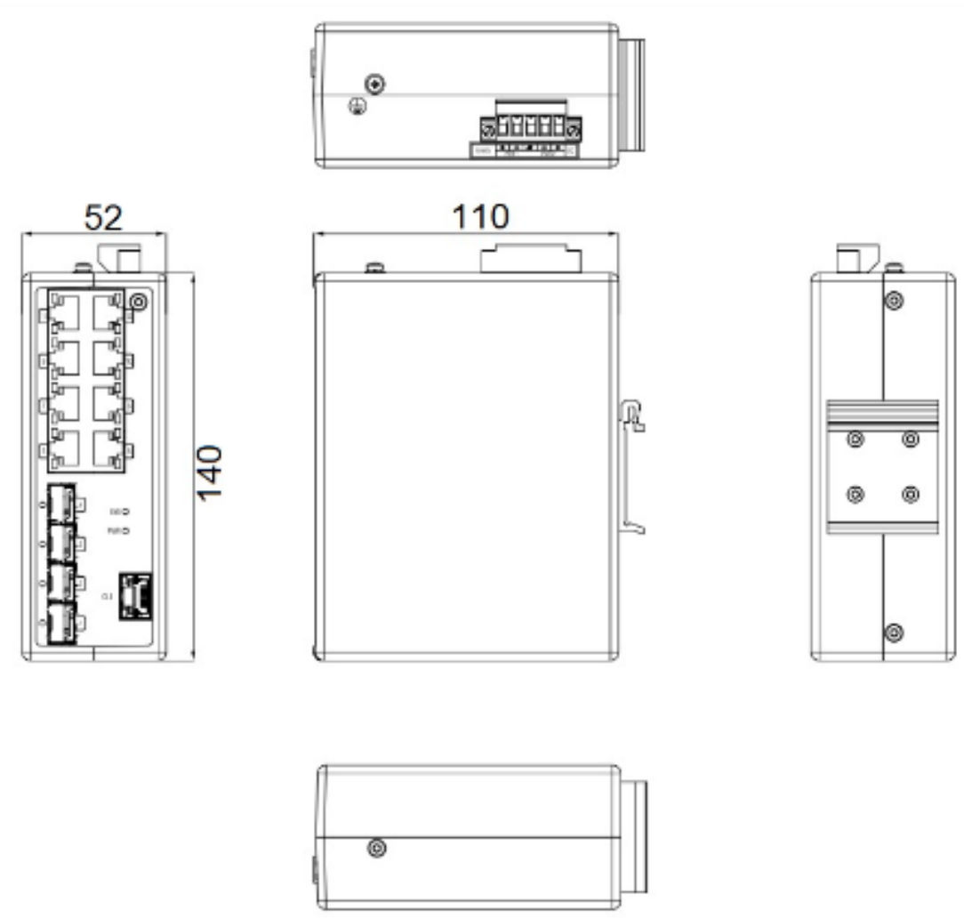
ISM7012D-P (52 × 140 × 110 mm)
